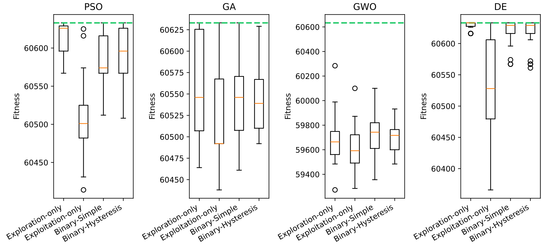
Fitness distribution across MH variants — mknapcb4[29] (opt=60633)
