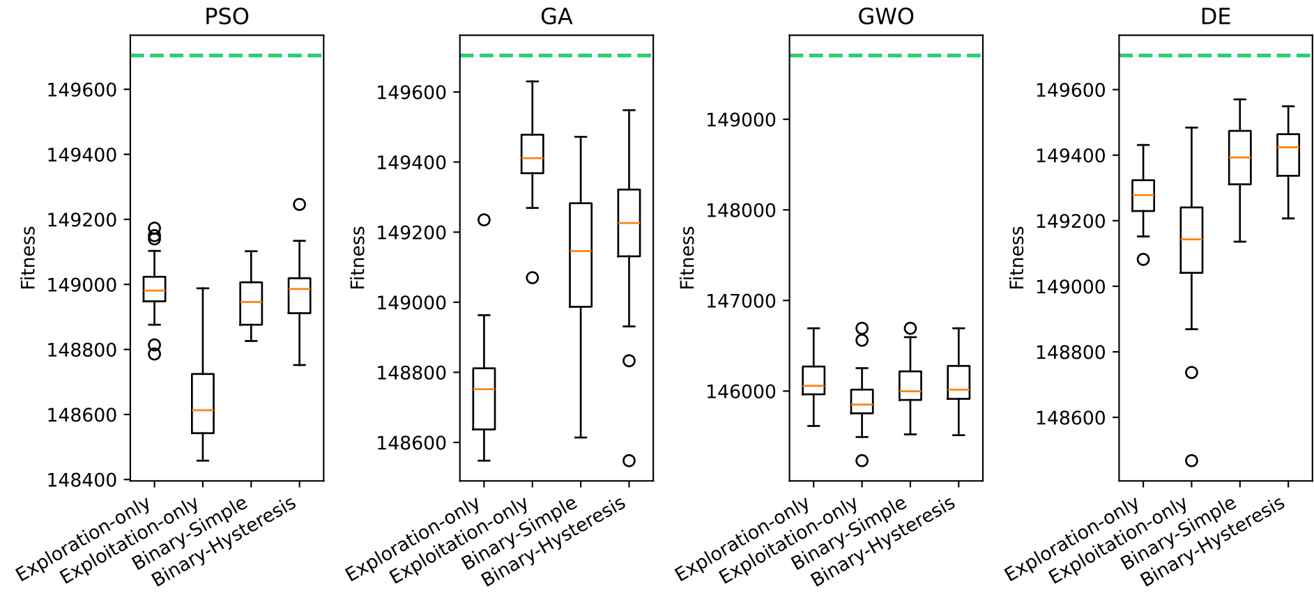
Fitness distribution across MH variants — mknapcb5[29] (opt=149704)
