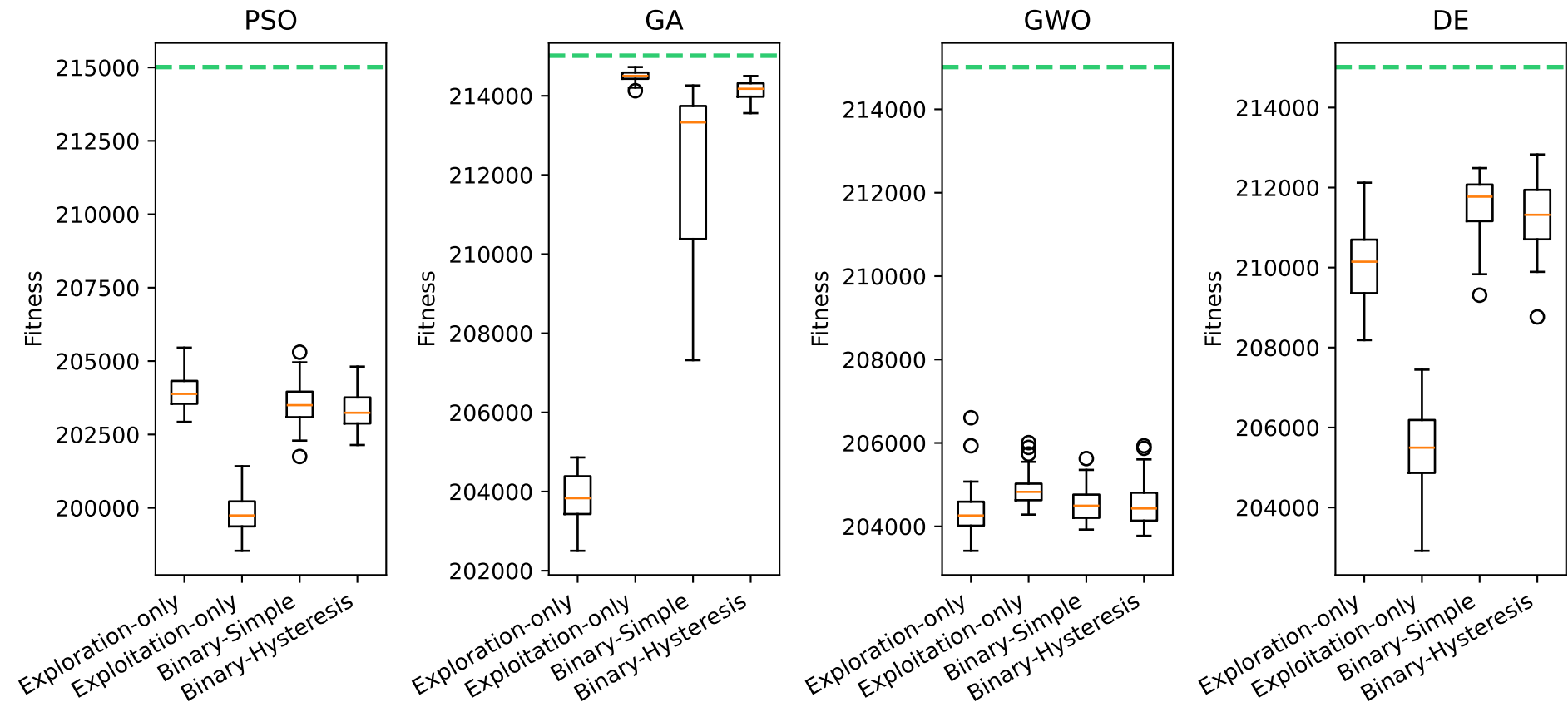
Fitness distribution across MH variants — mknapcb6[15] (opt=215013)
