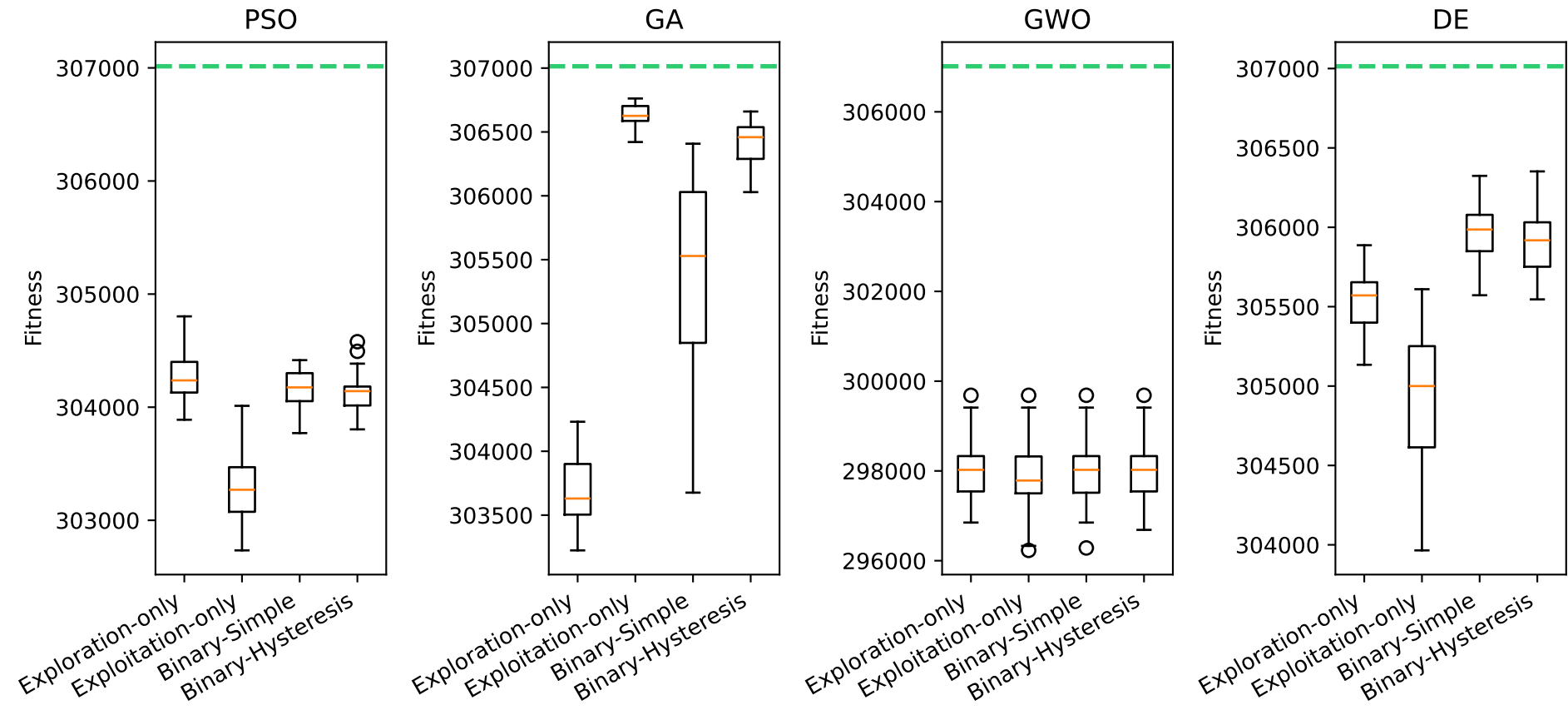
Fitness distribution across MH variants — mknapcb6[29] (opt=307014)
