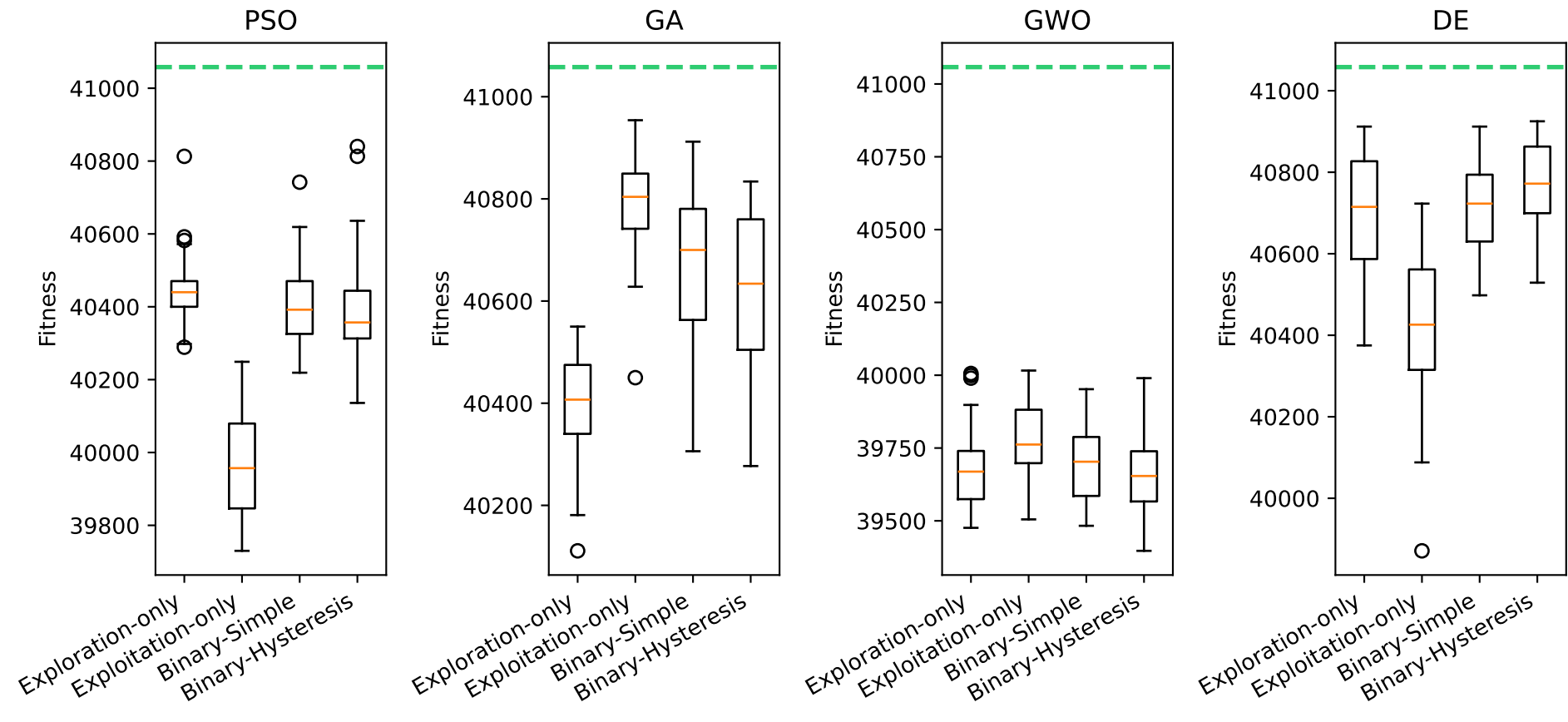
Fitness distribution across MH variants — mknapcb7[15] (opt=41058)
