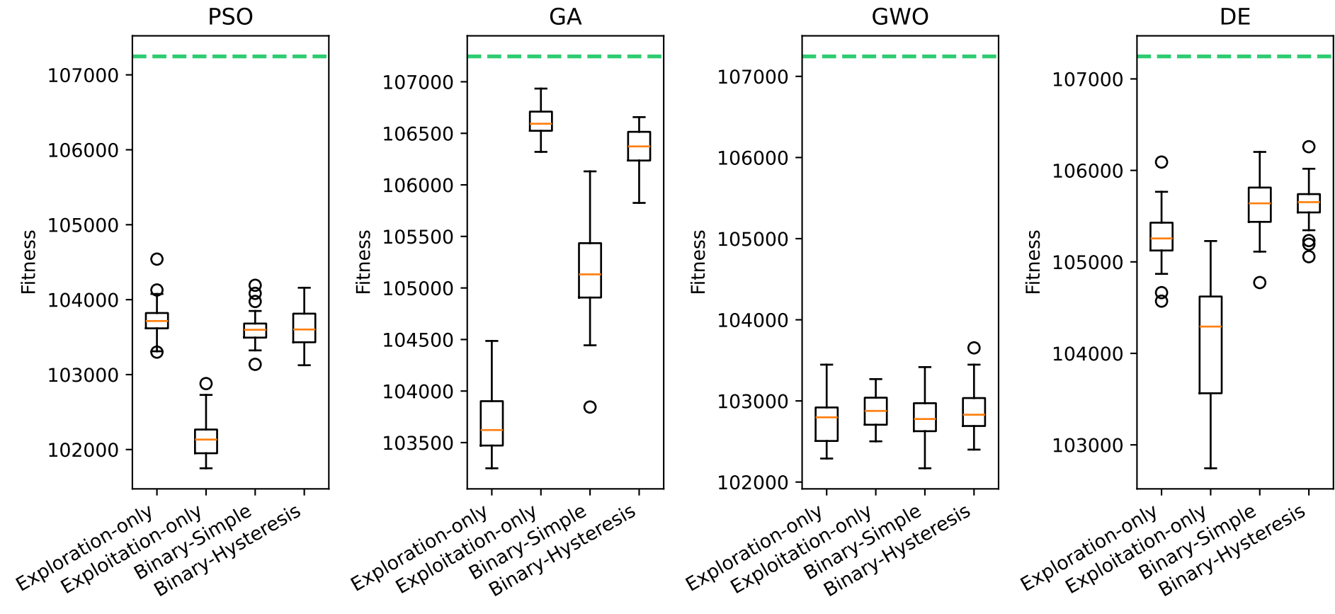
Fitness distribution across MH variants — mknapcb8[15] (opt=107246)
