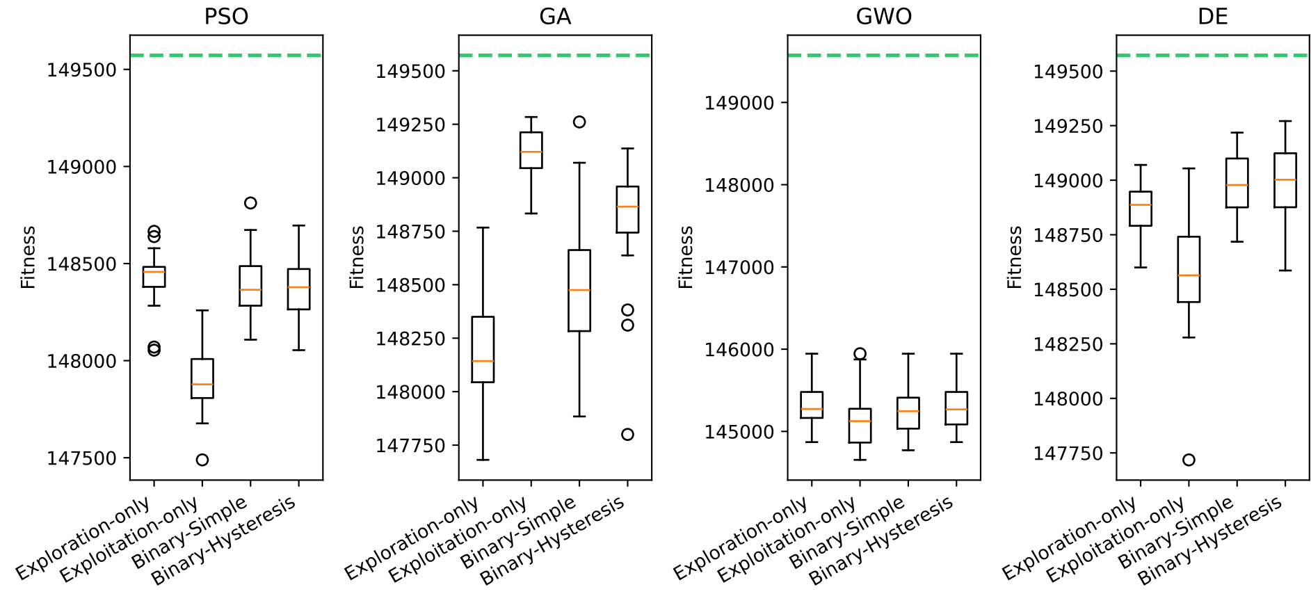
Fitness distribution across MH variants — mknapcb8[29] (opt=149572)
