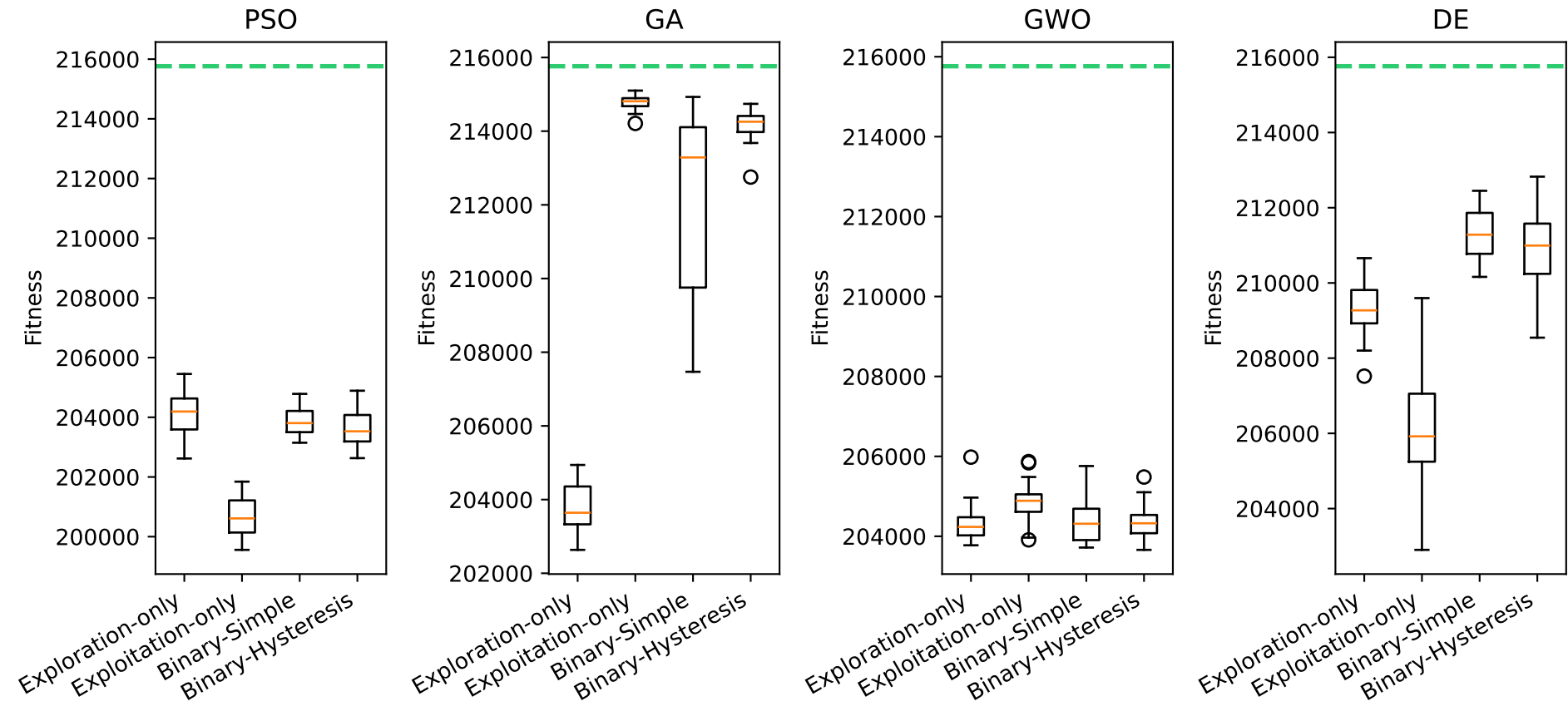
Fitness distribution across MH variants — mknapcb9[15] (opt=215762)
