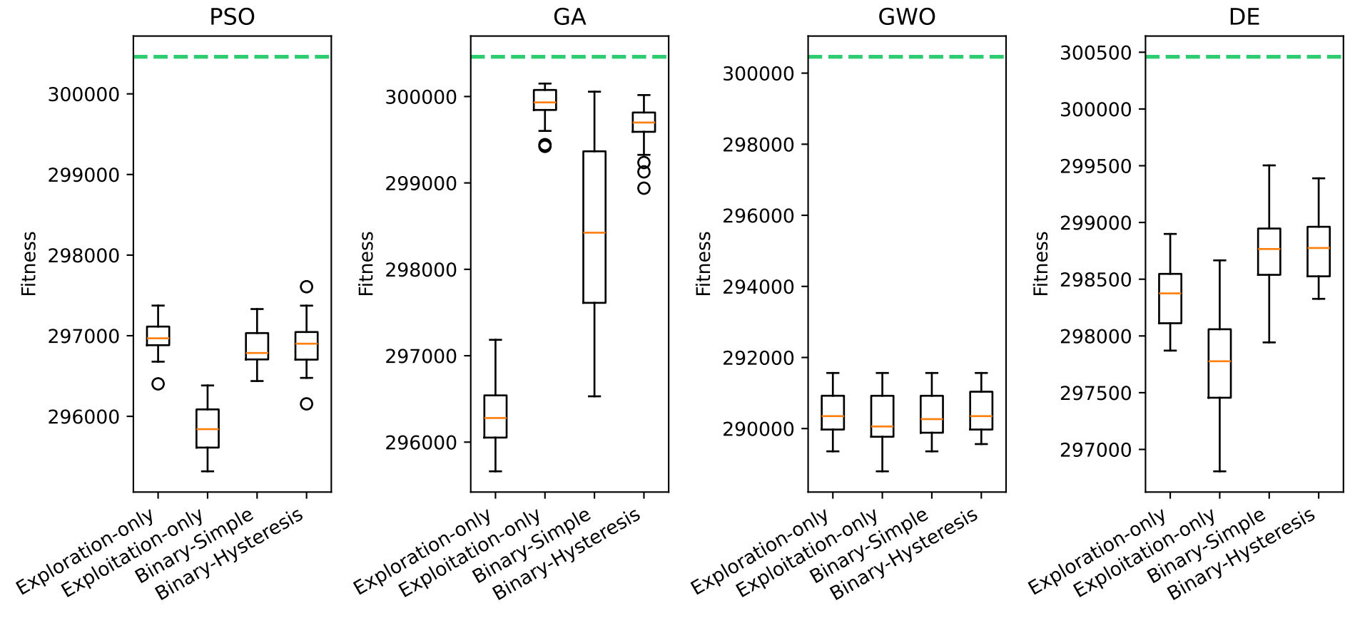
Fitness distribution across MH variants — mknapcb9[29] (opt=300460)
