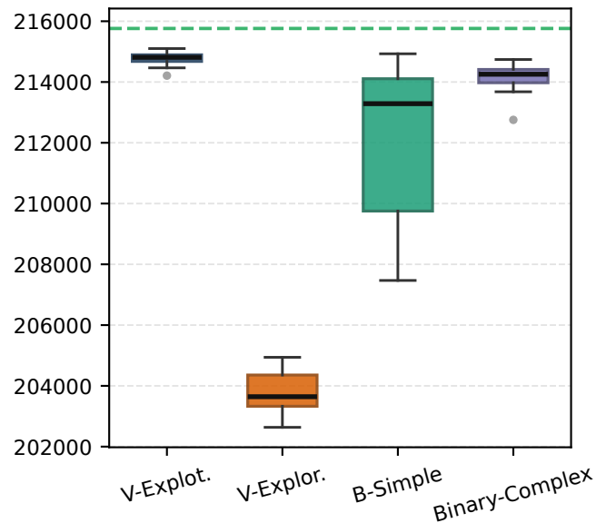
GA
