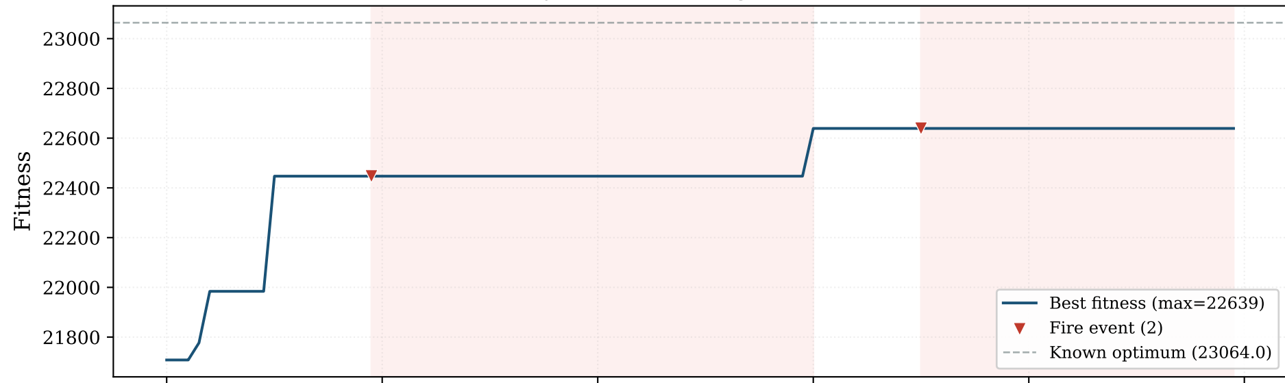
BinaryPSO — Convergence (seed=3)
