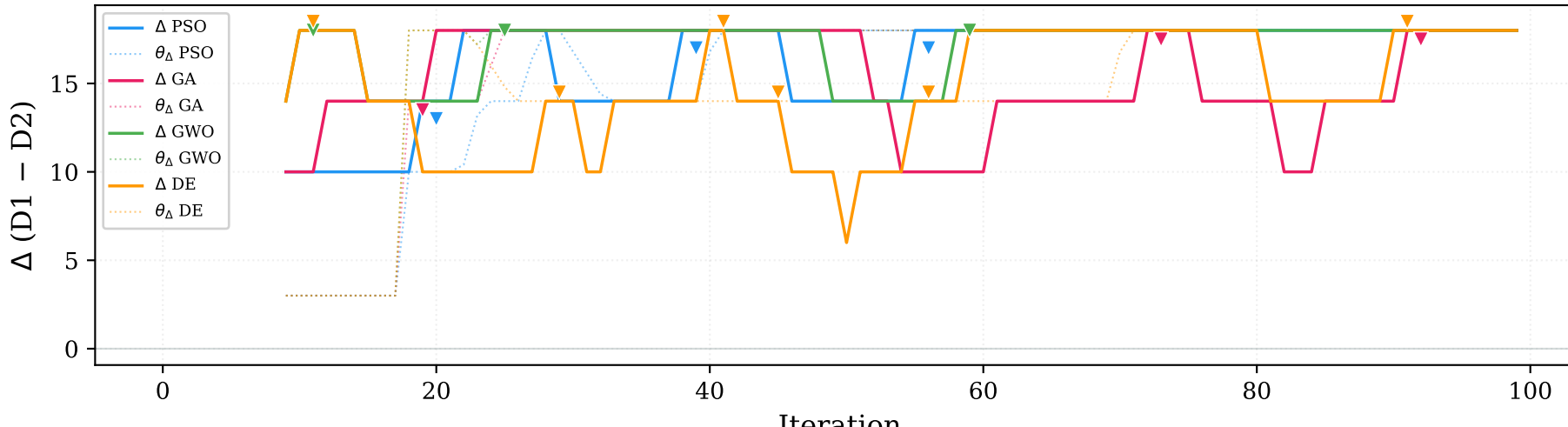
DTW Stagnation Signal — \Delta > 0 indicates stagnation
