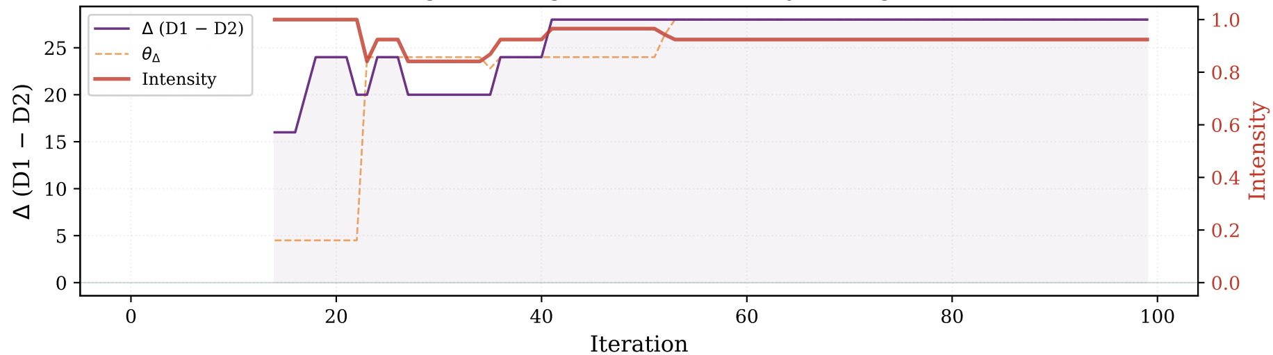
DTW Stagnation Signal — \Delta + Intensity (B1 sigmoid)
