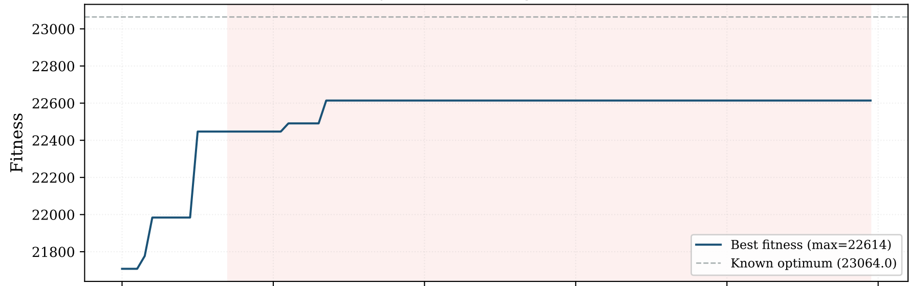
BinaryPSO — Convergence (seed=3)
