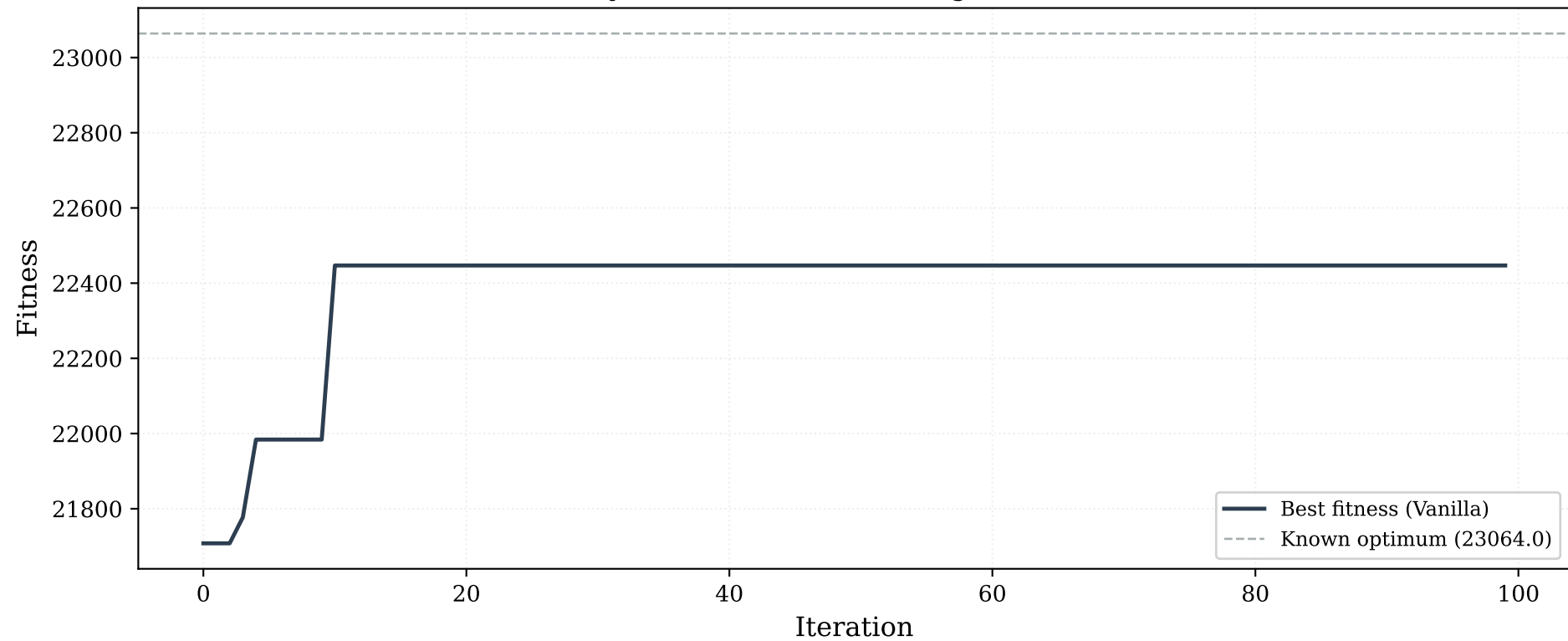
BinaryPSO Vanilla — Convergence (seed=3)
