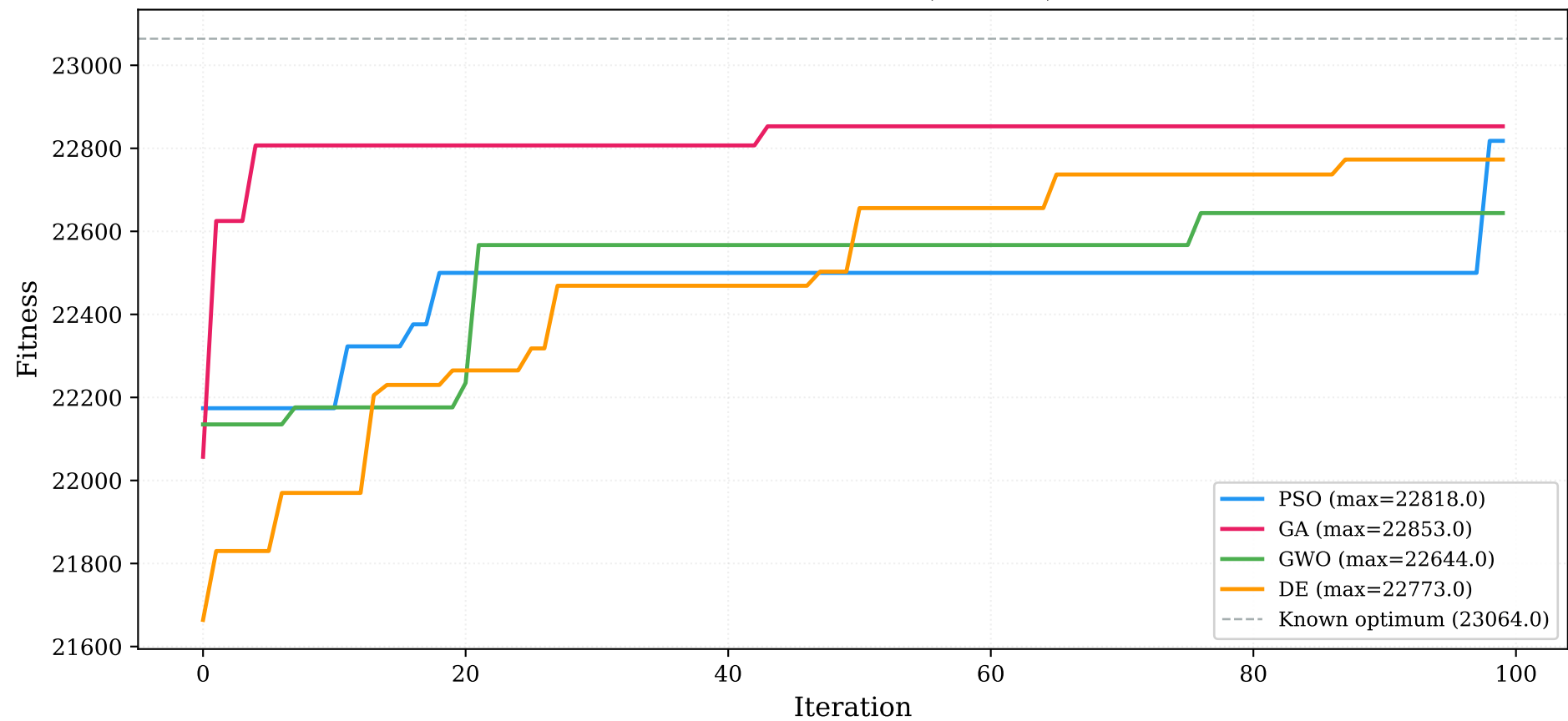
Vanilla — All MHs (seed=3)
