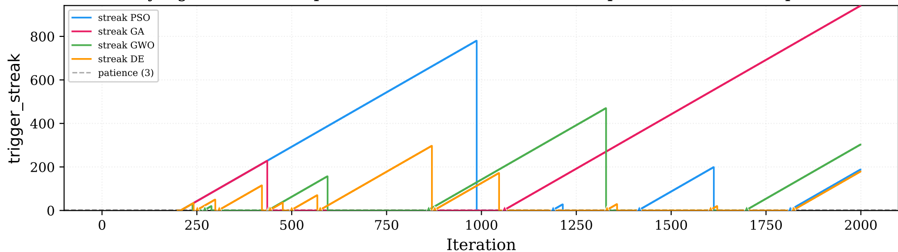
A4 entry signal — enter explore on sustained fire (streak \geq patience); exit on improvement
