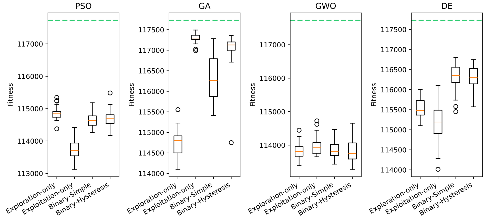
Fitness distribution across MH variants — mknapcb6[0] (opt=117726)
