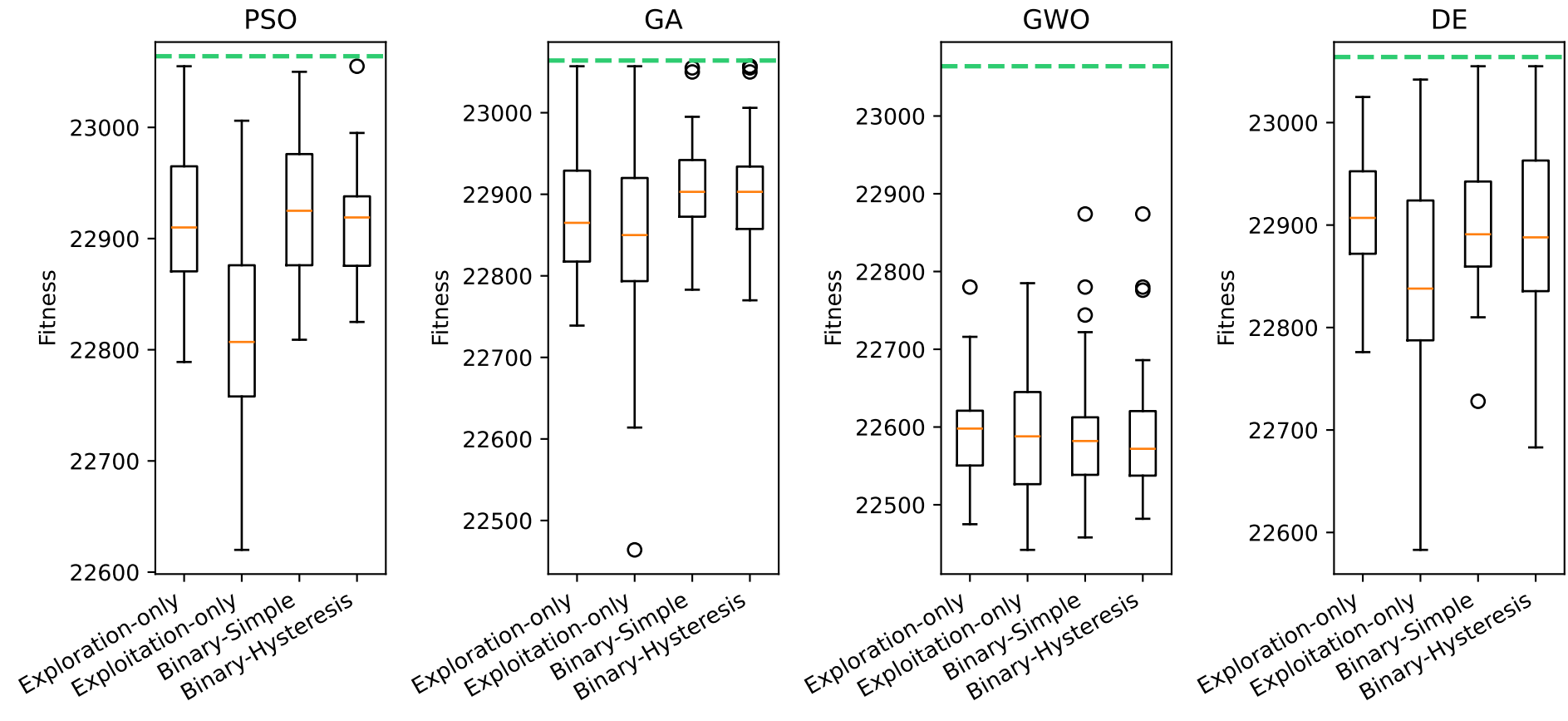
Fitness distribution across MH variants — mknapcb4[0] (opt=23064)
