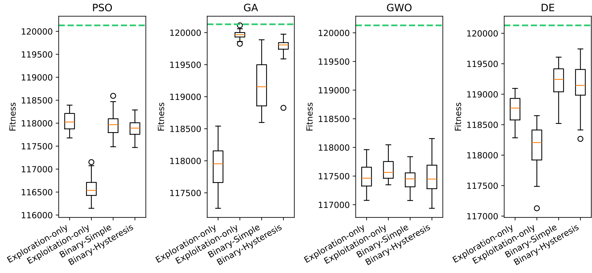
Fitness distribution across MH variants — mknapcb3[0] (opt=120130)
