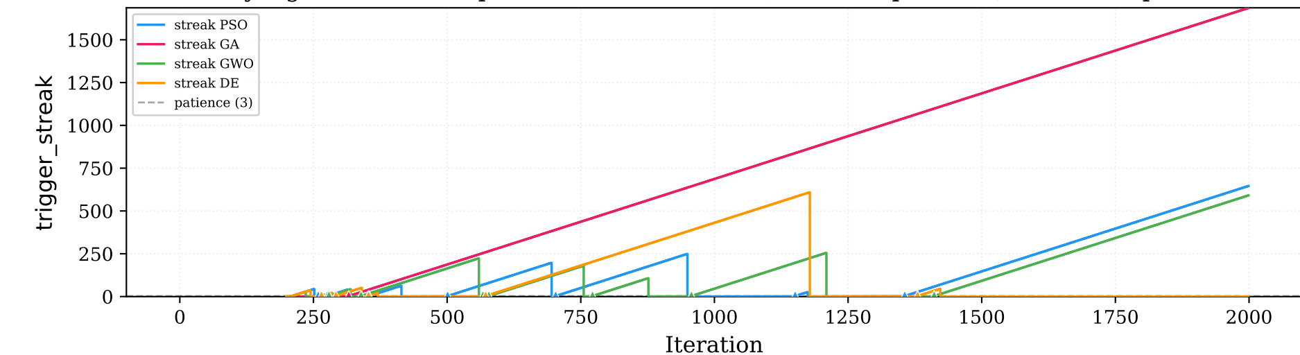
A4 entry signal — enter explore on sustained fire (streak \geq patience); exit on improvement
