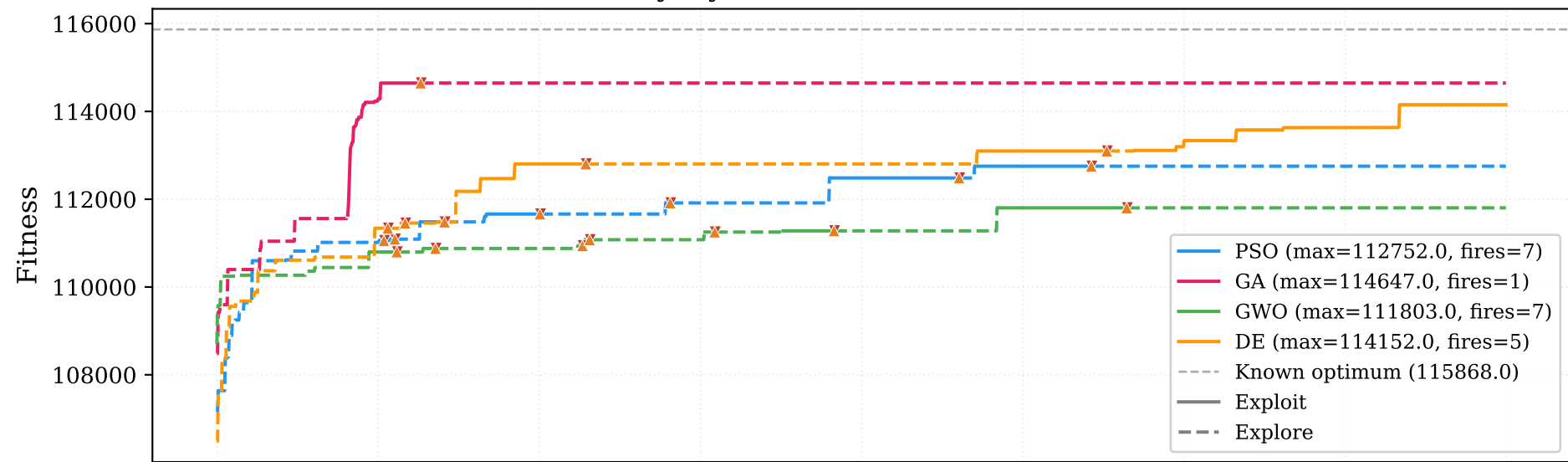
Binary-Hysteresis — All MHs (seed=1)
