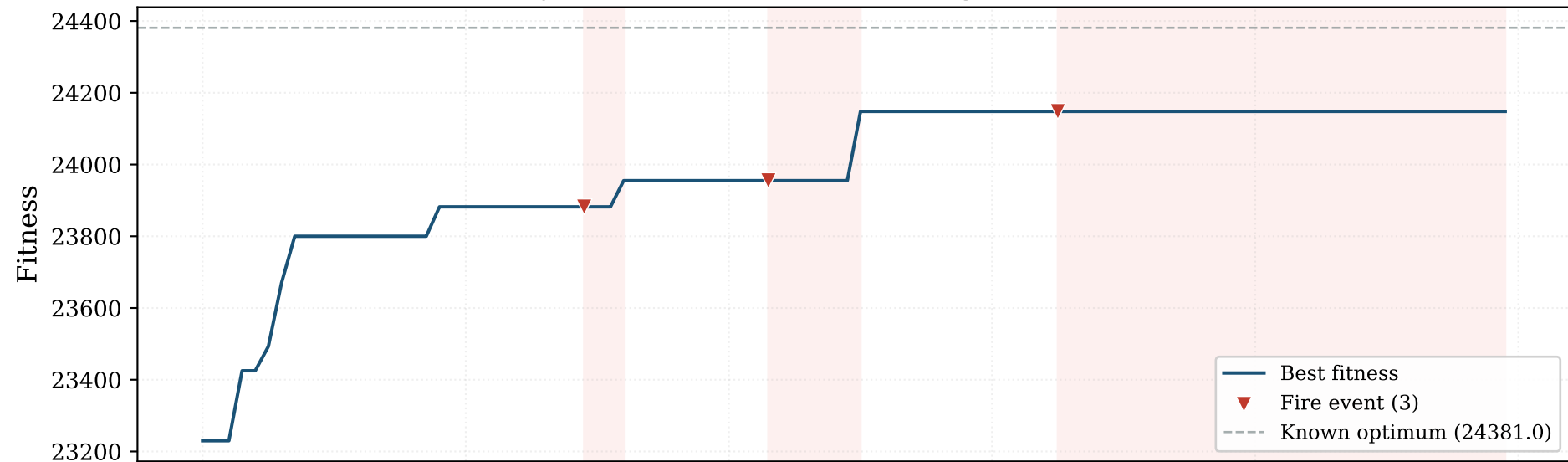
BinaryPSO + DTW Fire — Convergence (seed=None)
