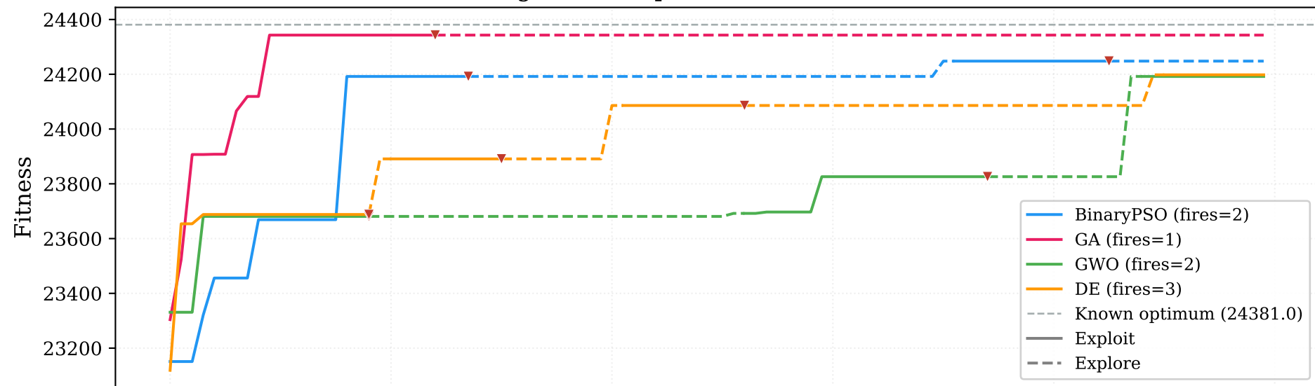
Convergence Comparison — All MHs (seed=3)
