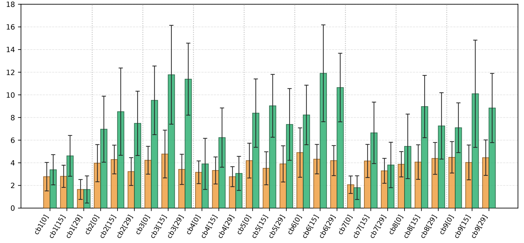
BDE
