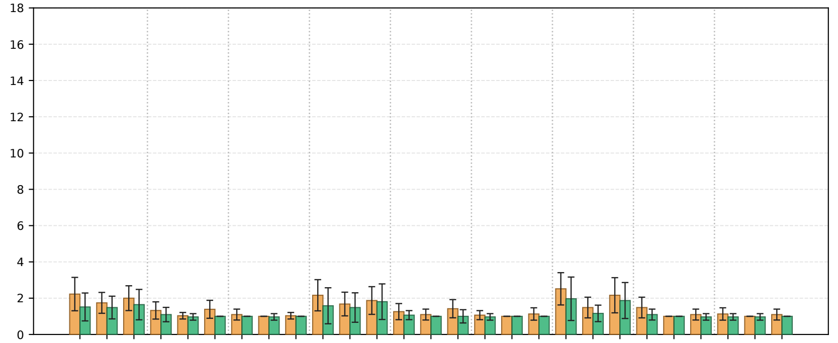
BDE
