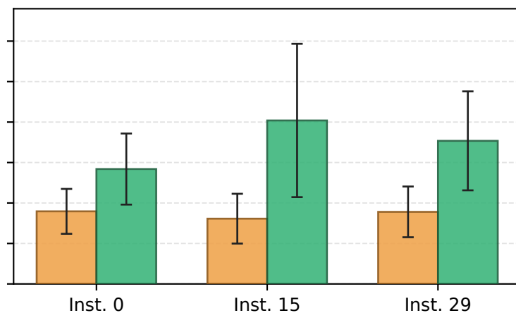
BDE
