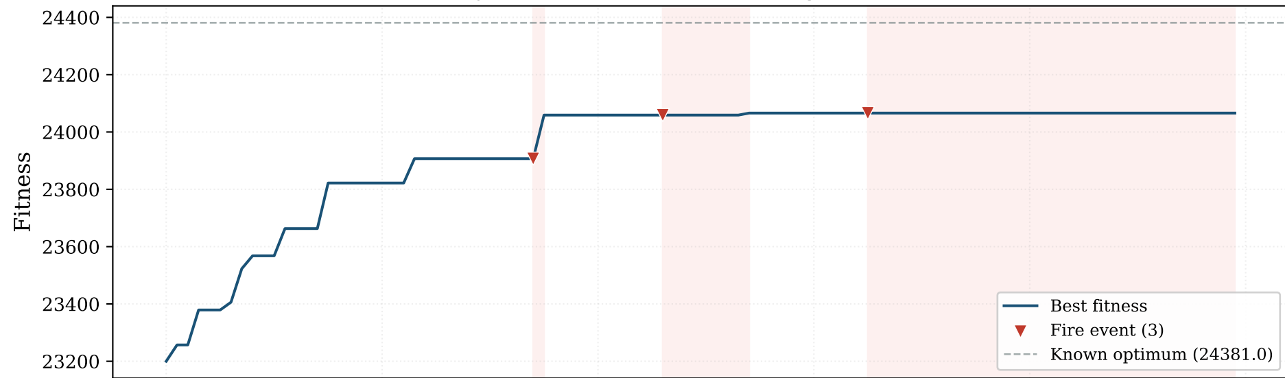
BinaryDE + DTW Fire — Convergence (seed=3)
