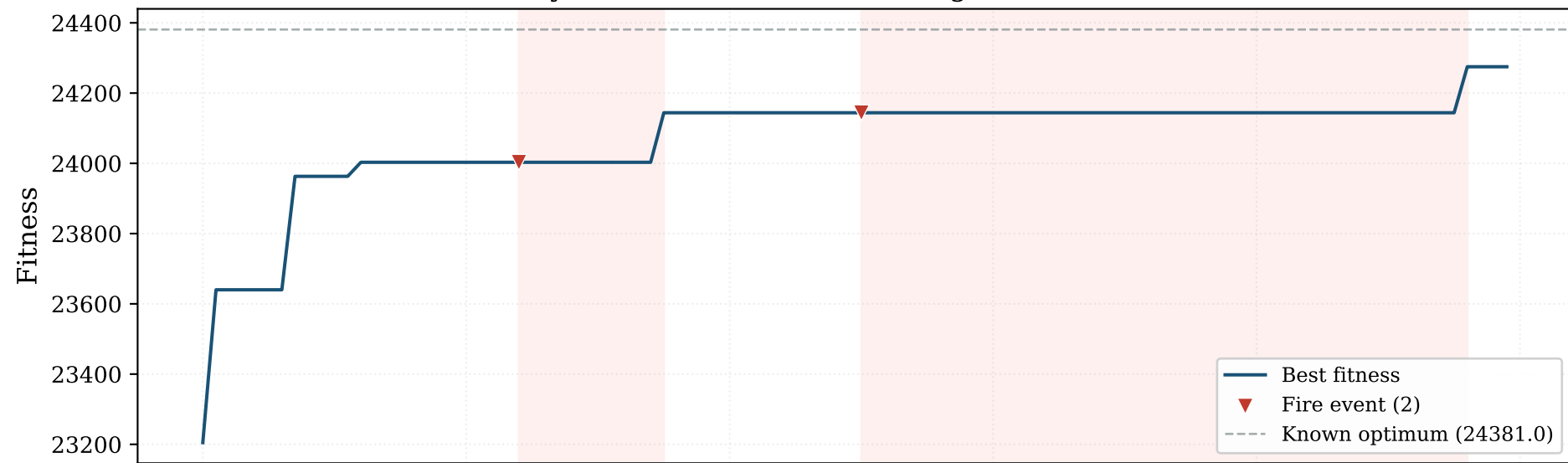
BinaryDE + DTW Fire — Convergence (seed=None)
