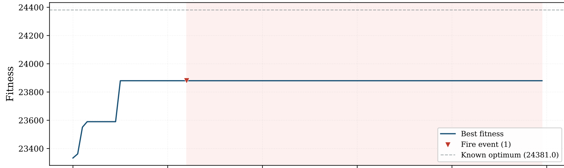
BinaryGWO + DTW Fire — Convergence (seed=None)
