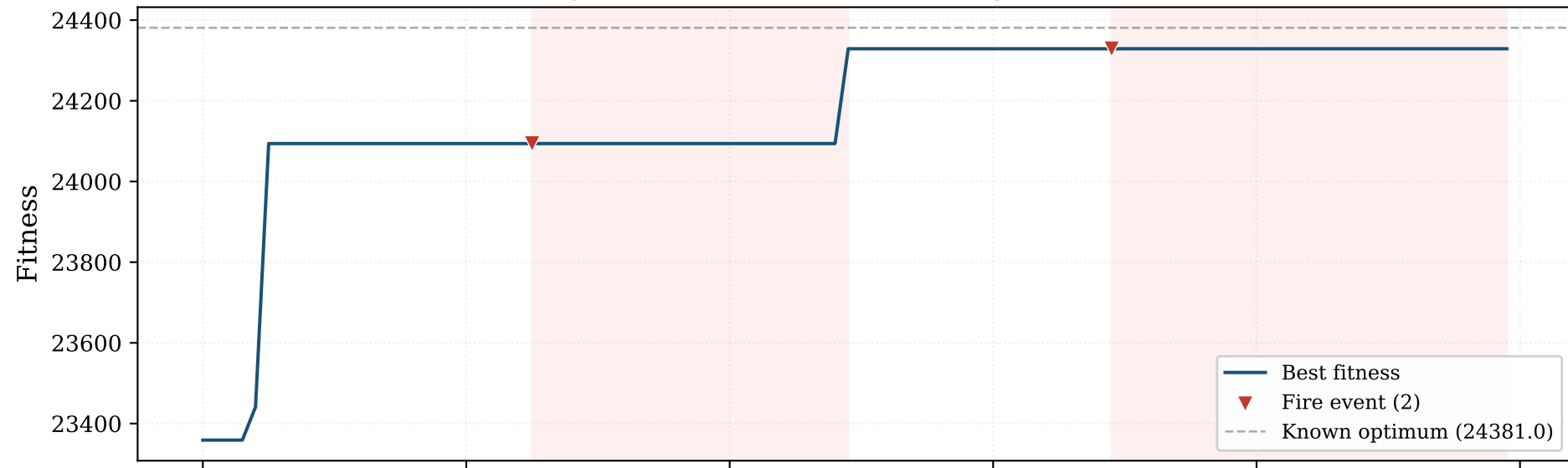
BinaryPSO + DTW Fire — Convergence (seed=3)
