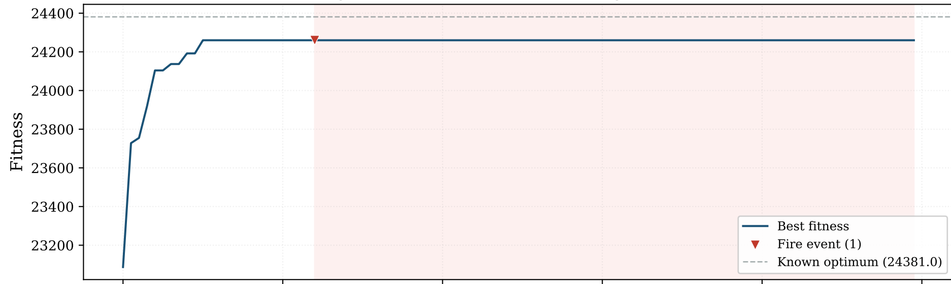
GeneticAlgorithm + DTW Fire — Convergence (seed=None)
