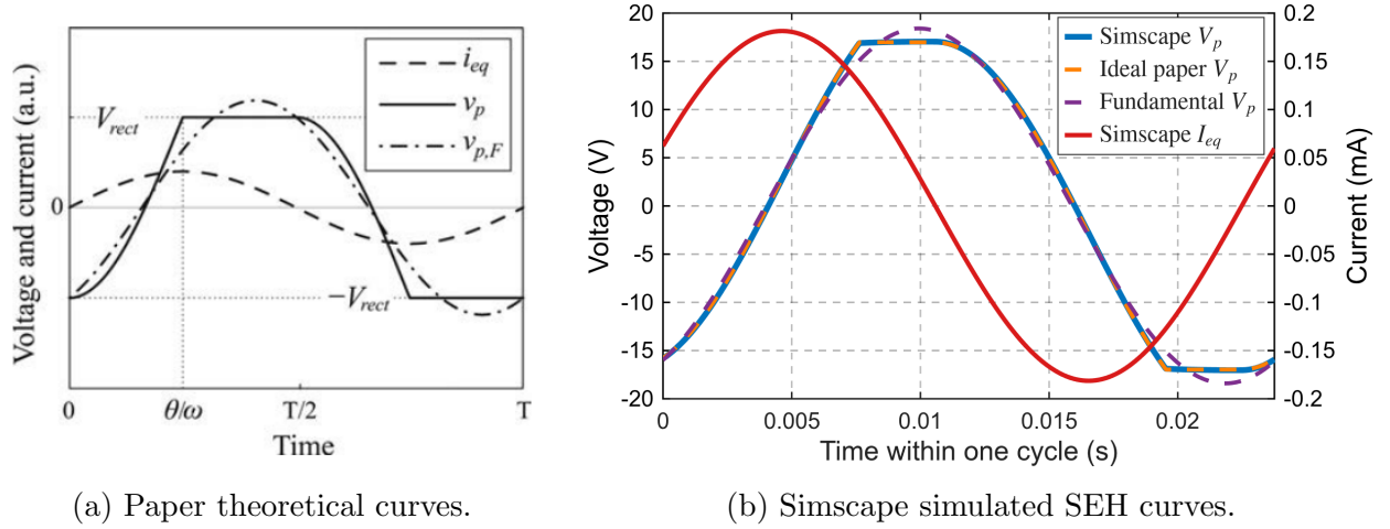
Figure 2.4: Simulation results look identical to paper graph and numerical paper equations waveform. The measured solid blue V_p from simulation is directly matched with the dotted blue ideal paper V_p , Eq. (2.29) and the red I_{eq} curve being out of phase like in the paper graph. Figure (a) taken from [1, Fig. 3].
