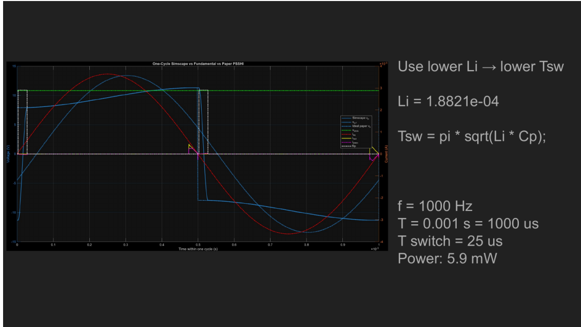
Figure 4.3: High-frequency P-SSHI result after reducing L_i so that the LC inversion occupies a small fraction of the 1000 Hz cycle.
