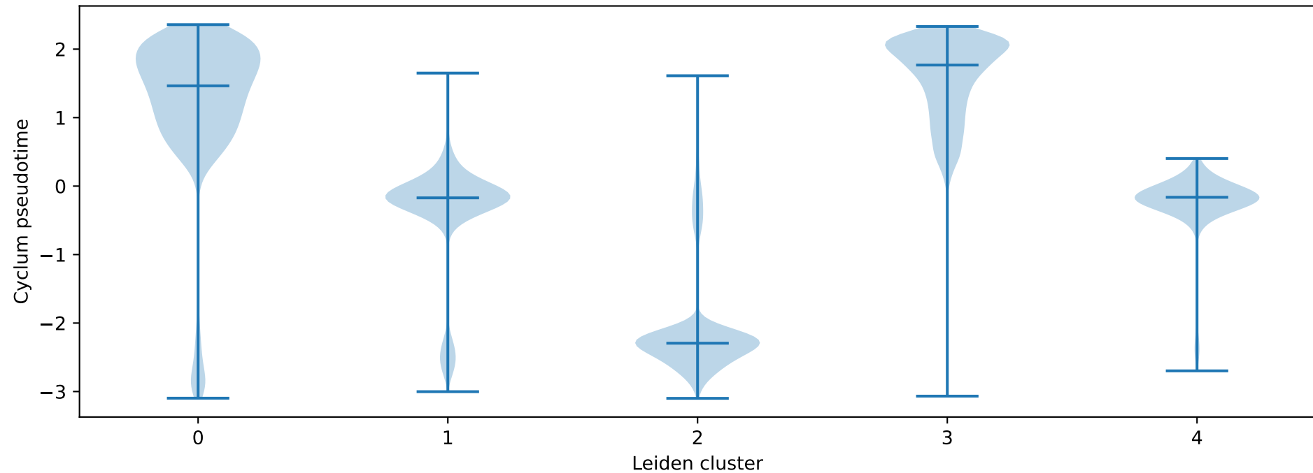
Cyclum pseudotime distribution per Leiden cluster
