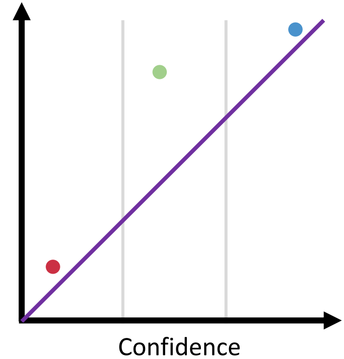
Over-confident
