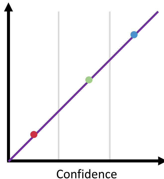
Calibrated
