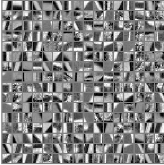
256 Learned Dictionary Atoms (K-SVD, Camera Man, \sigma = 25 )
