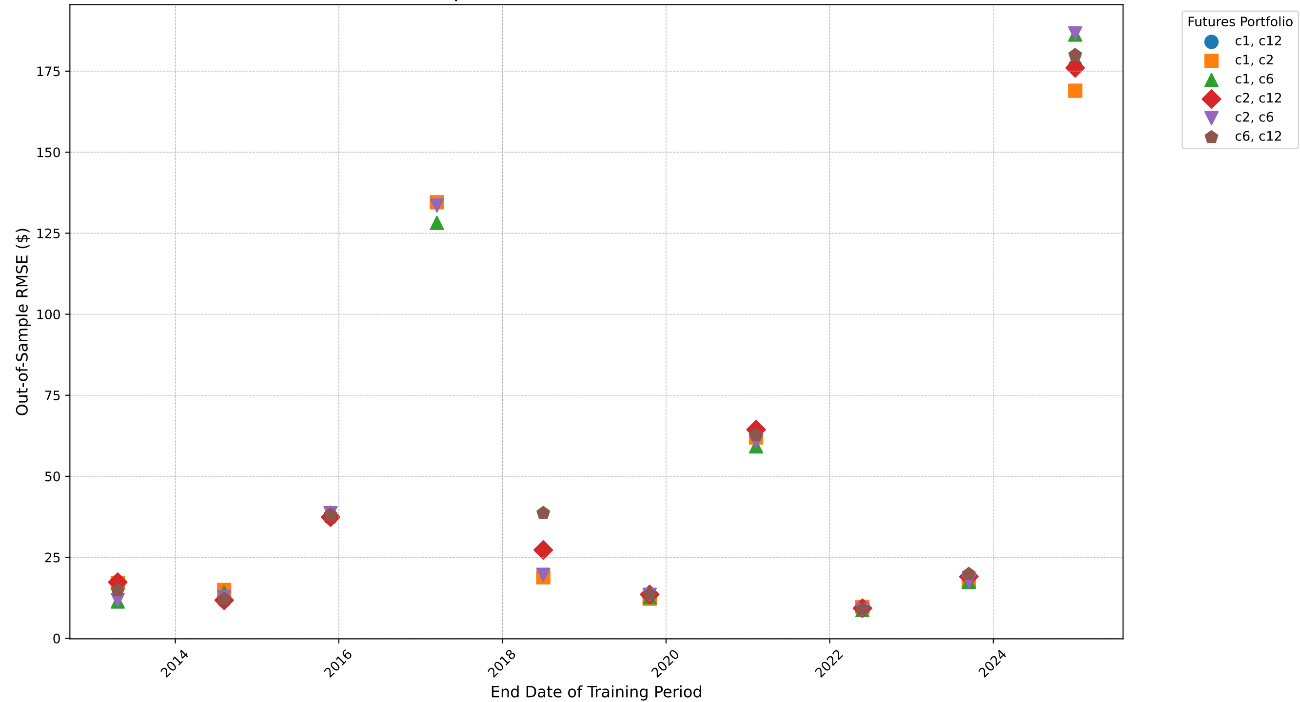
Out-of-Sample RMSE Across Cross-Validation Folds
