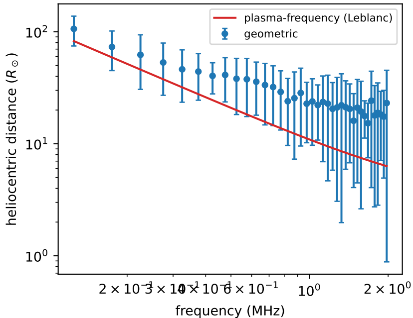
Geometric vs plasma distance
