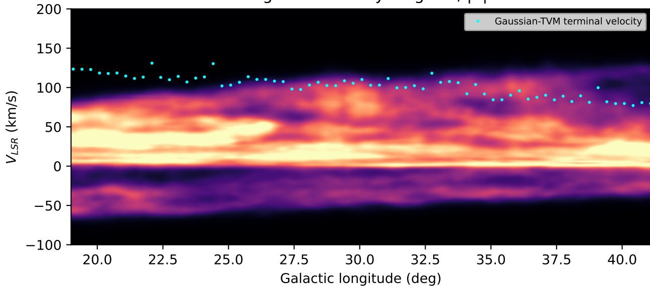
HI4PI longitude-velocity diagram, |b| < 3^\circ
