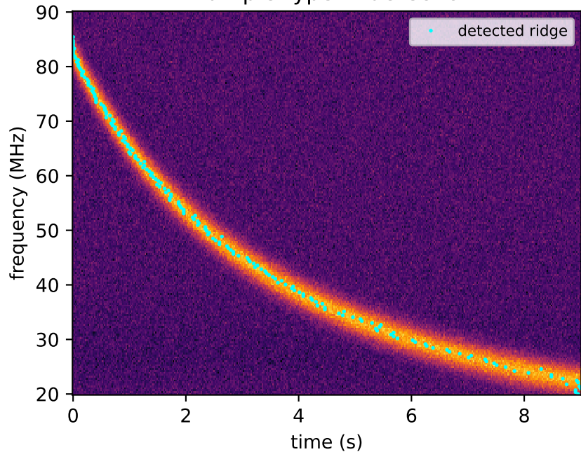
Example type III detection
