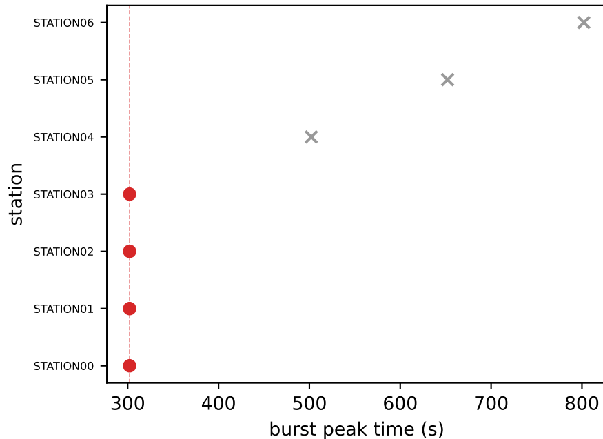
Coincidence QC: 1 confirmed
