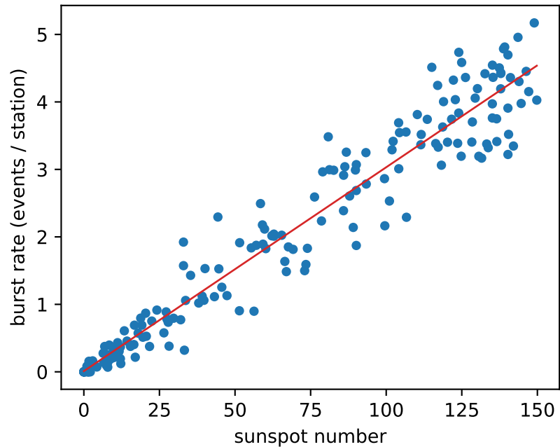
Rate vs activity
