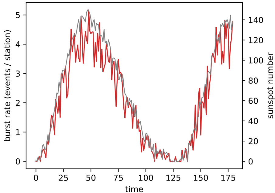
Occurrence vs solar cycle
