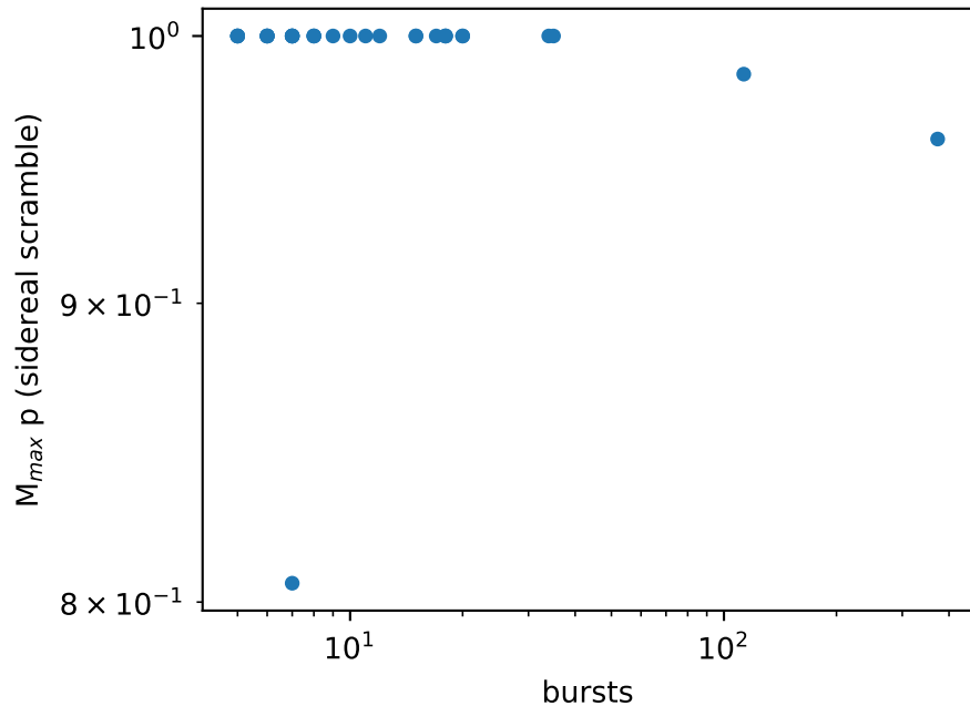
Recurring-delay search
