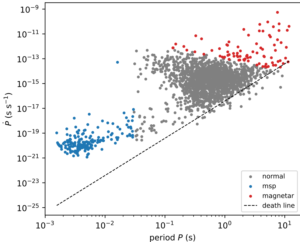
The pulsar P--Pdot diagram
