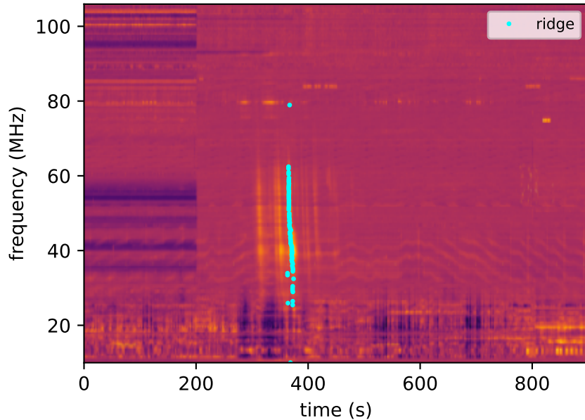
Type III dynamic spectrum
