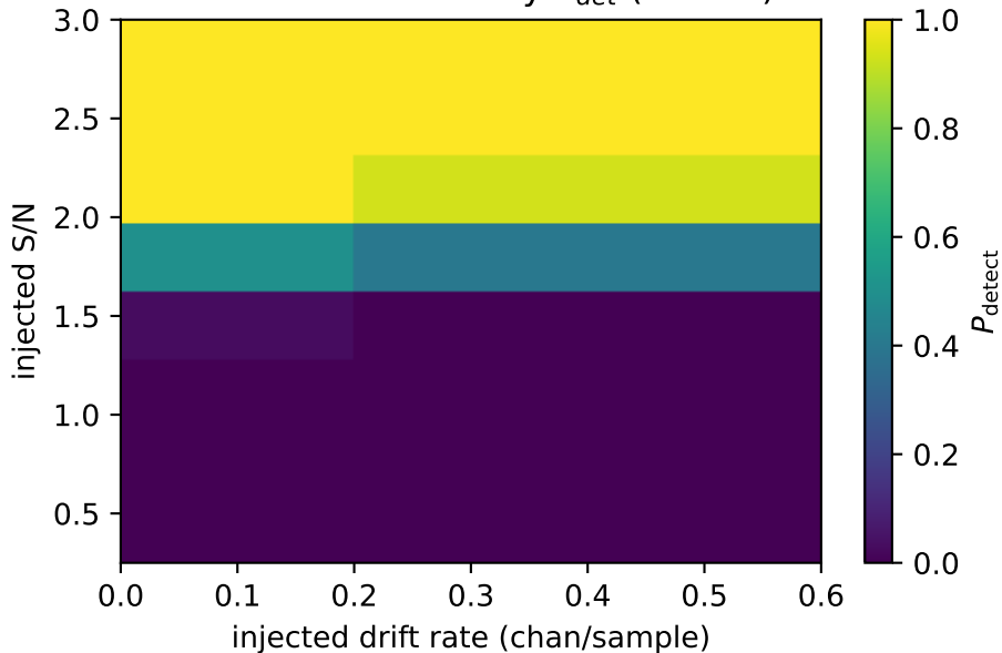
Drift-search recovery P_{det} (FPR=0)
