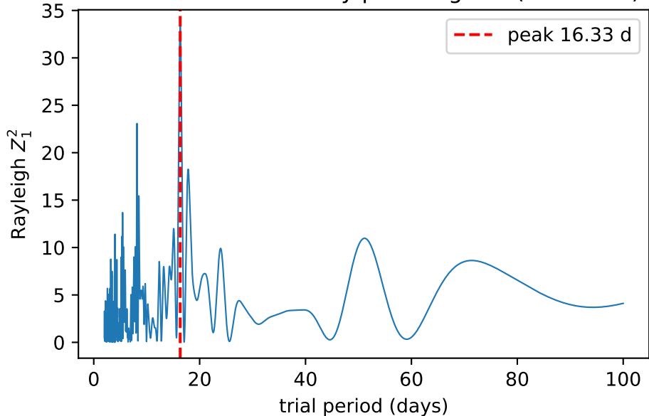
FRB20180916B activity periodogram (19 bursts)
