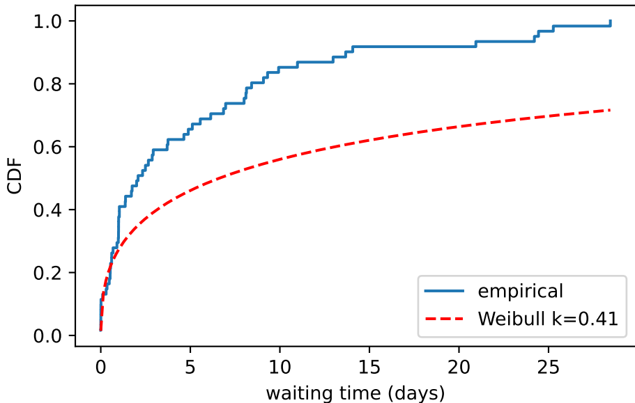
Repeater inter-burst wait times
