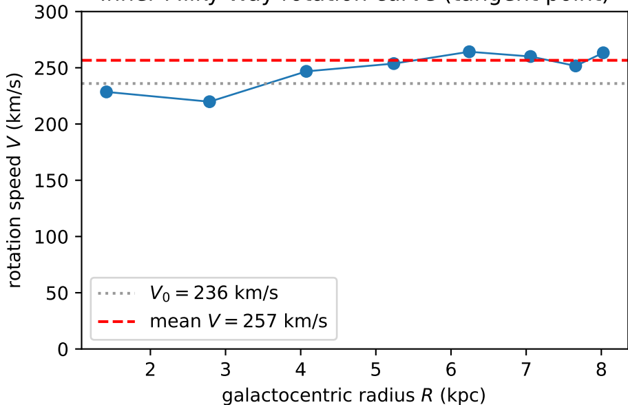
Inner Milky Way rotation curve (tangent point)
