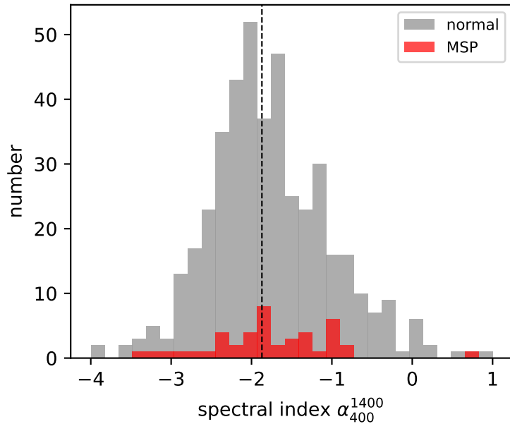
Pulsar spectra
