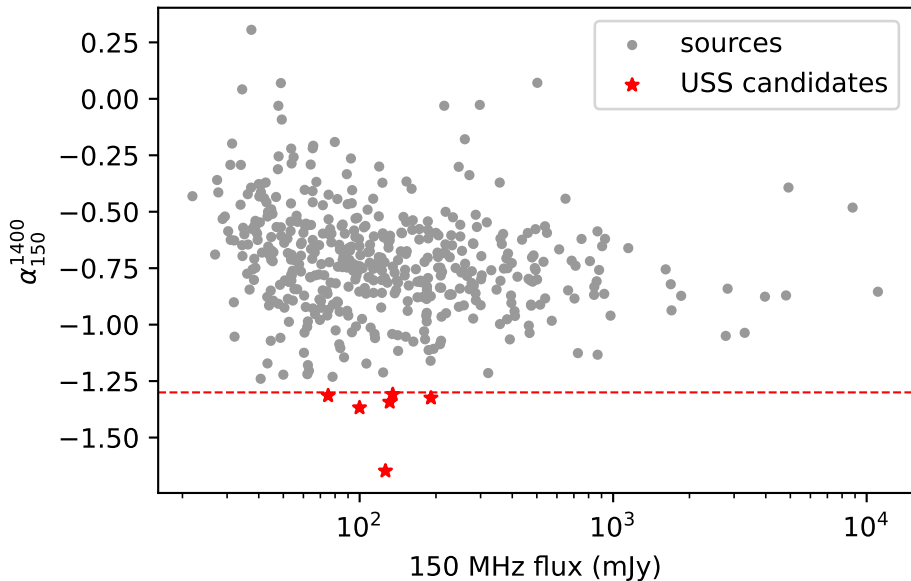
USS candidates vs flux
