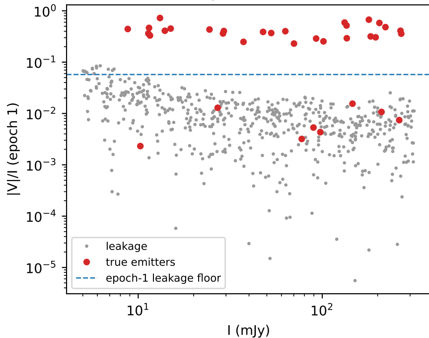
Per-epoch selection
