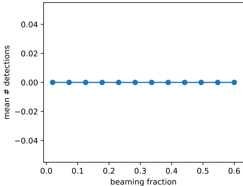
Prior-predictive
