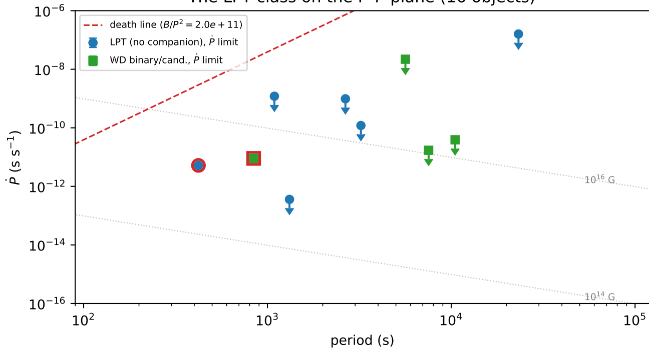
The LPT class on the P-\dot{P} plane (16 objects)
